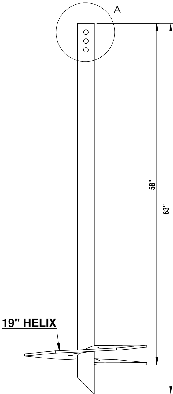
1 2.5" SCH40 SINGLE HELIX 1:10
