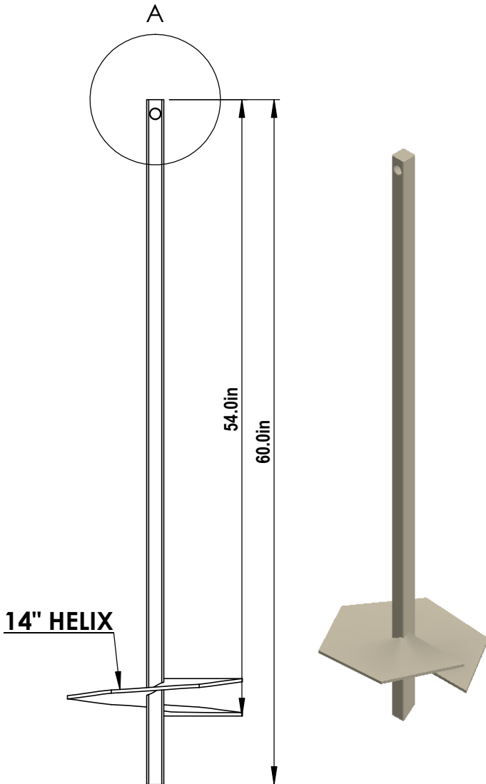
1 1.5" RCS SINGLE HELIX 1" = 1' 0"
