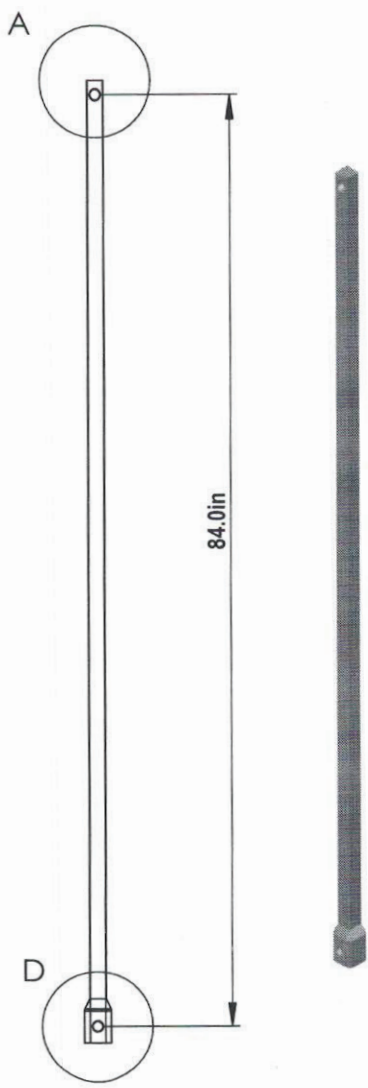
2 1.5" RCS EXTENSION 3/4" = 1' 0"
